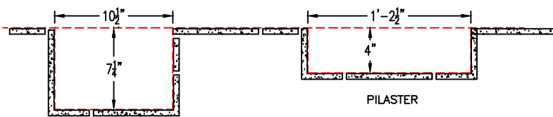
PILASTER
